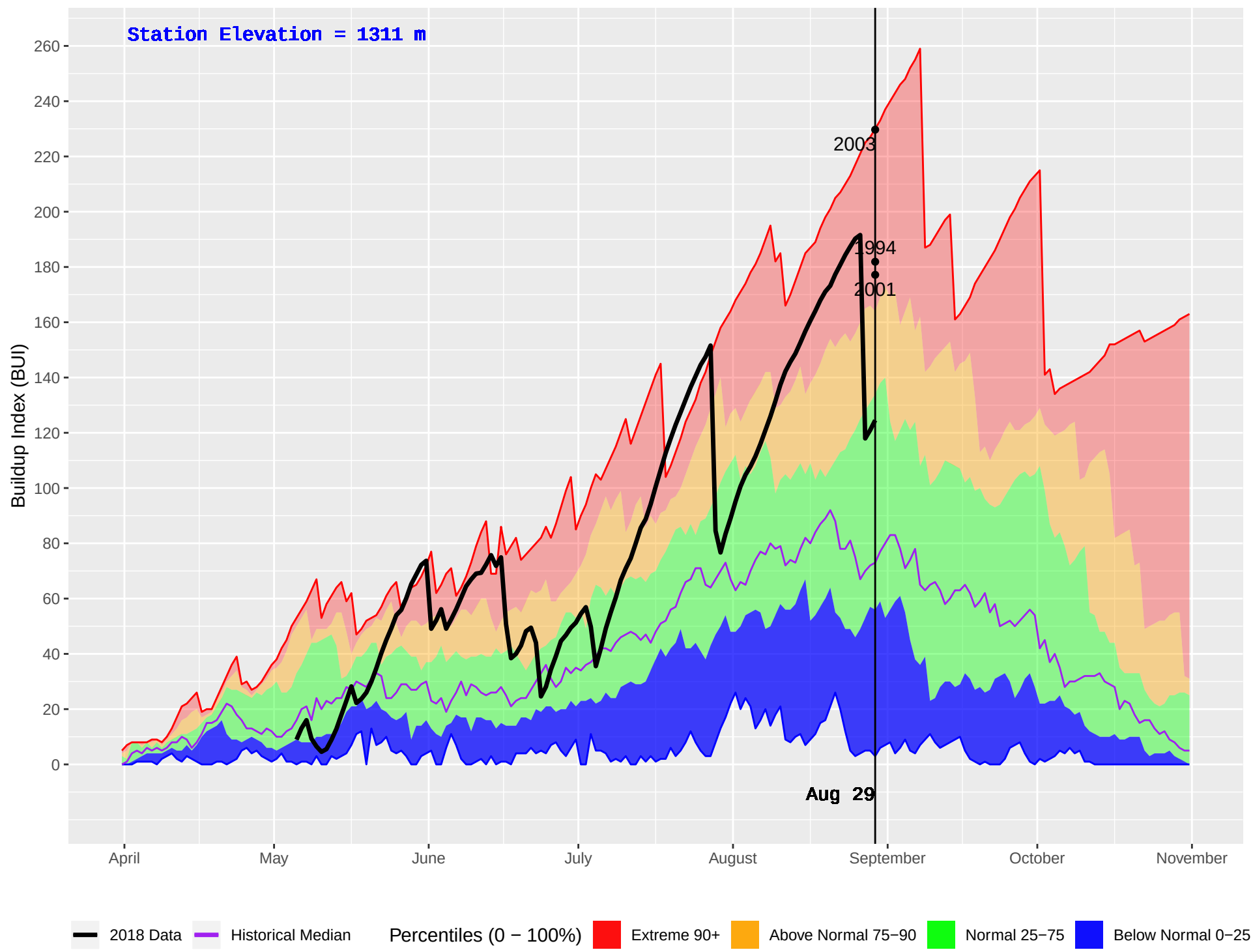
FLATHEAD 2 (418) : Historical (1986–2016) and Current (2018) Daily Buildup Index (BUI)
