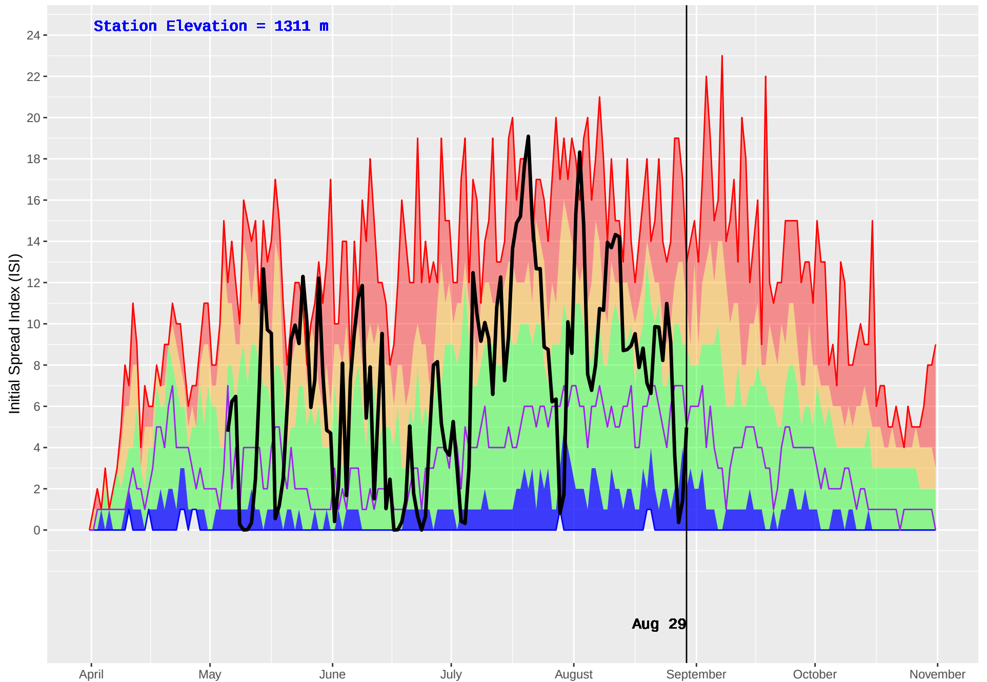
FLATHEAD 2 (418) : Historical (1986–2016) and Current (2018) Daily Initial Spread Index (ISI)
