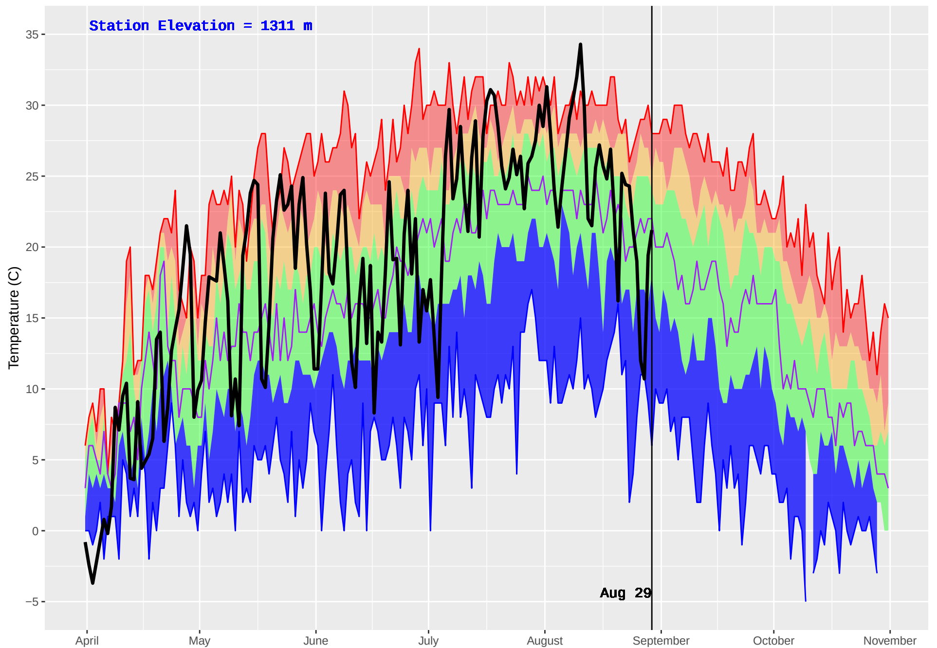
FLATHEAD 2 (418) : Historical (1986–2016) and Current (2018) Daily Temperature
